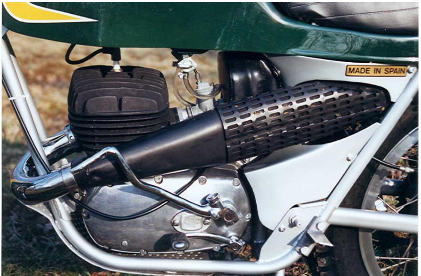
Bore is 72mm and stroke is 60mm. Engine has electronic ignition
